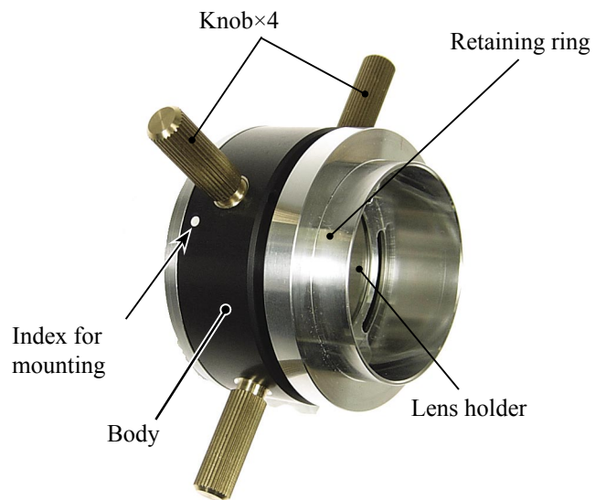
5th lens -G alignment tool ( ★ J11328)
