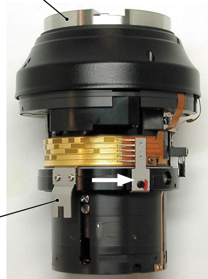
Focus coupling key
