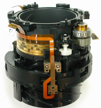
Fixed tube unit
