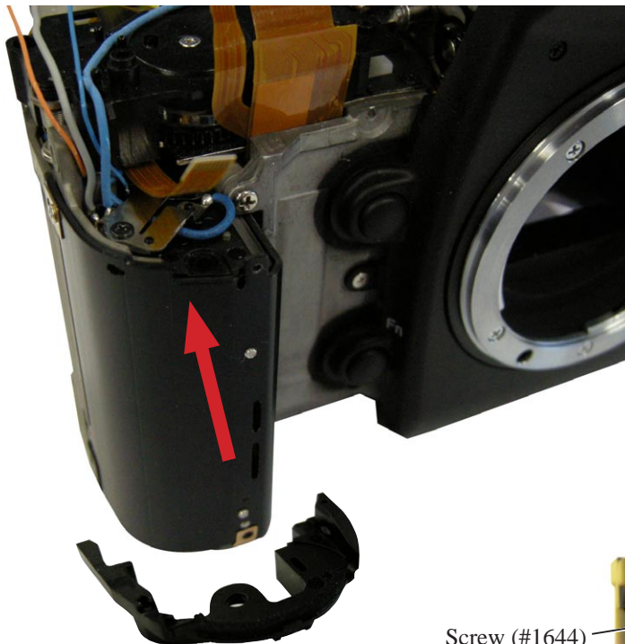
Grip-supporting mold (#58)
