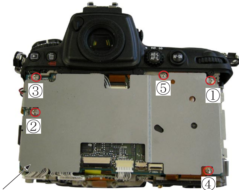
DG shield plate unit (#B683)
