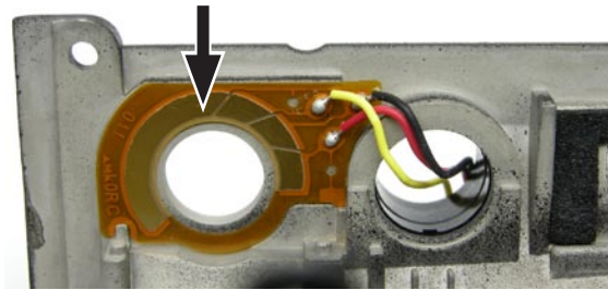
Metering mode FPC (#5028)
