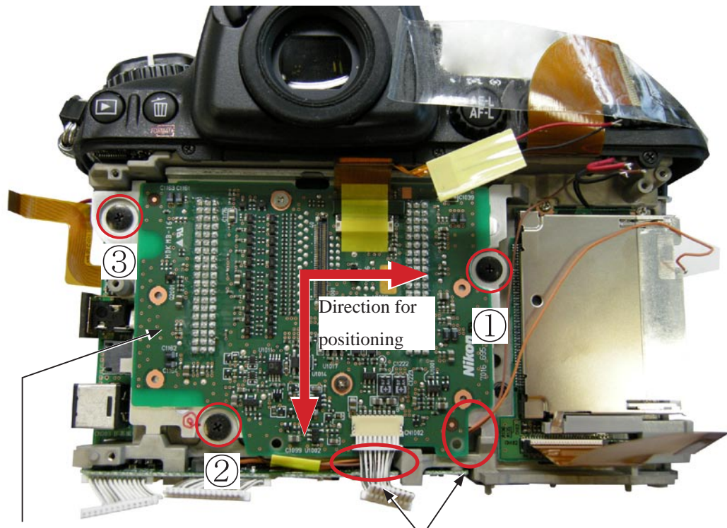
Image sensor unit (#B20521)
